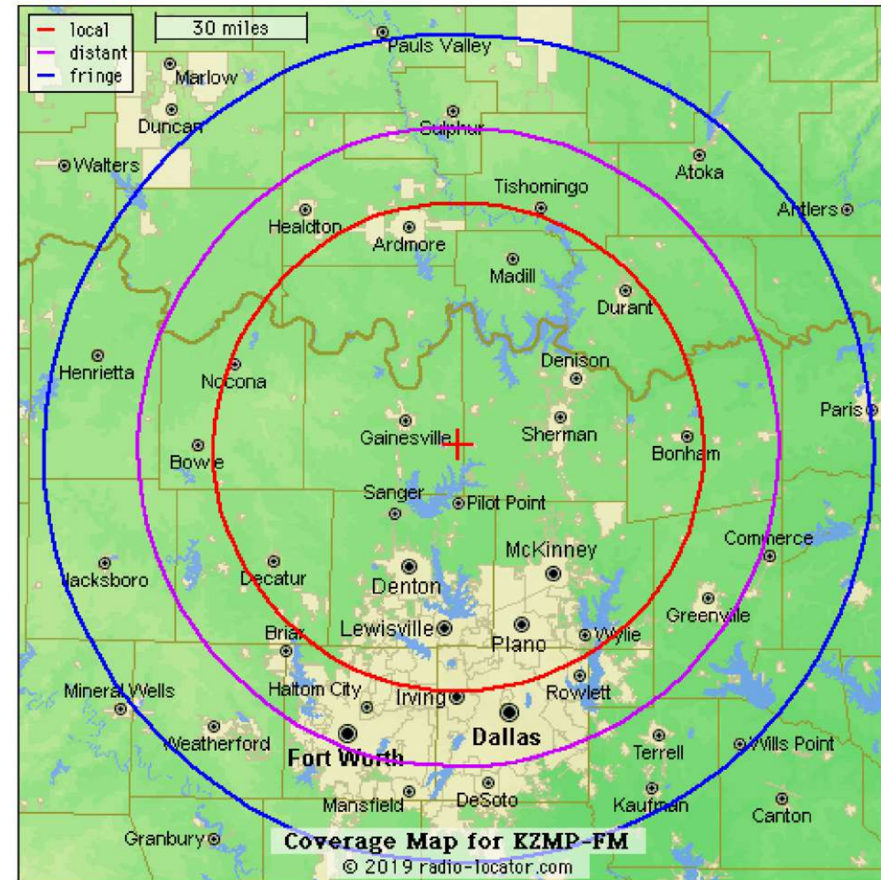
Coverage Area for KZMP 104.9 FM , Pilot Point, TX
